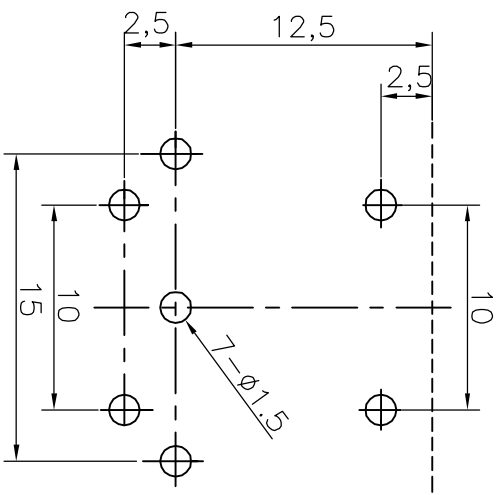
P.C.B. HOLE LAYOUT (BOTTOM VIEW)
